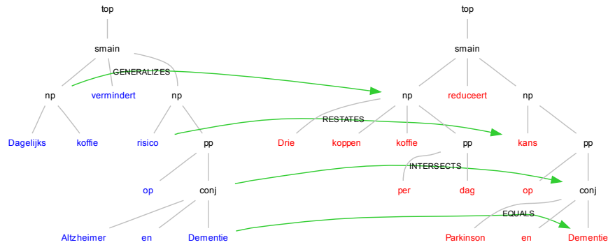
Figure 1: Example of two (partially) aligned syntactic trees
